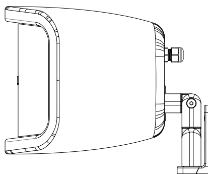
Figure 5.6a: Vertical bracket mounting
