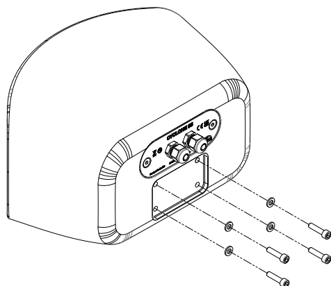
Figure 5.16: Bolt removal
