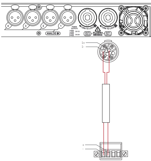
Figure 4.11: Bias Q5
