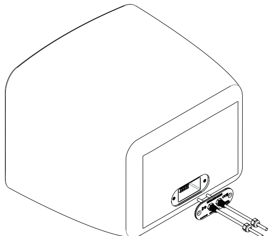
Figure 4.4: Cable connection
