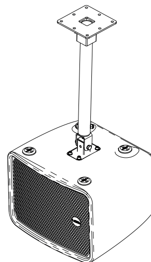
Figure 5.12: Loudspeaker positioning
