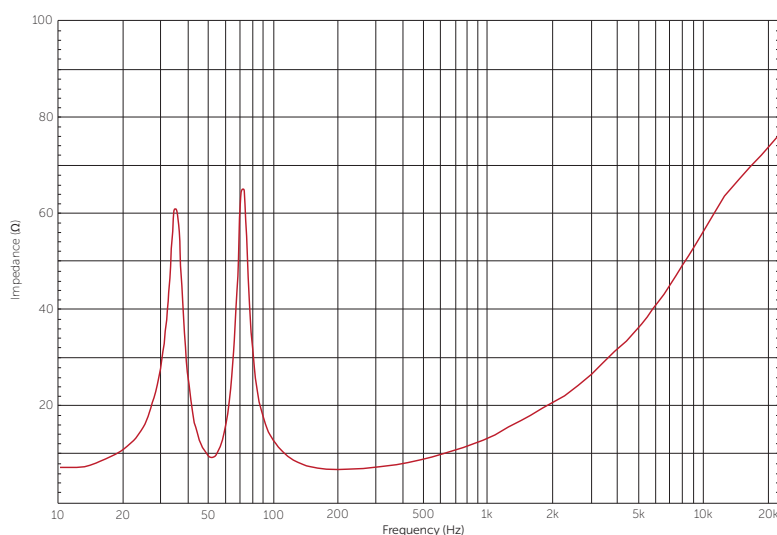
Figure 3.1: Impedance graph
